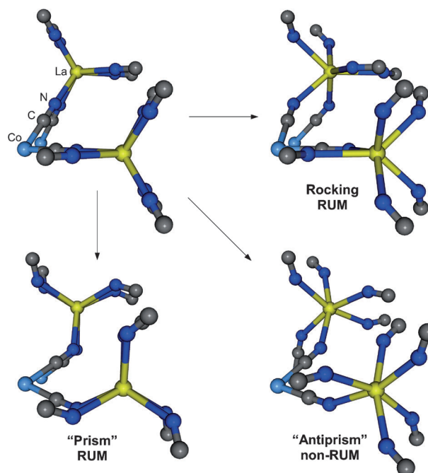
Figure 4. Three low-energy modes contributing to NTE in LaCo(CN) 6 , viewed along the c -axis. See the Supporting Information for animations.
